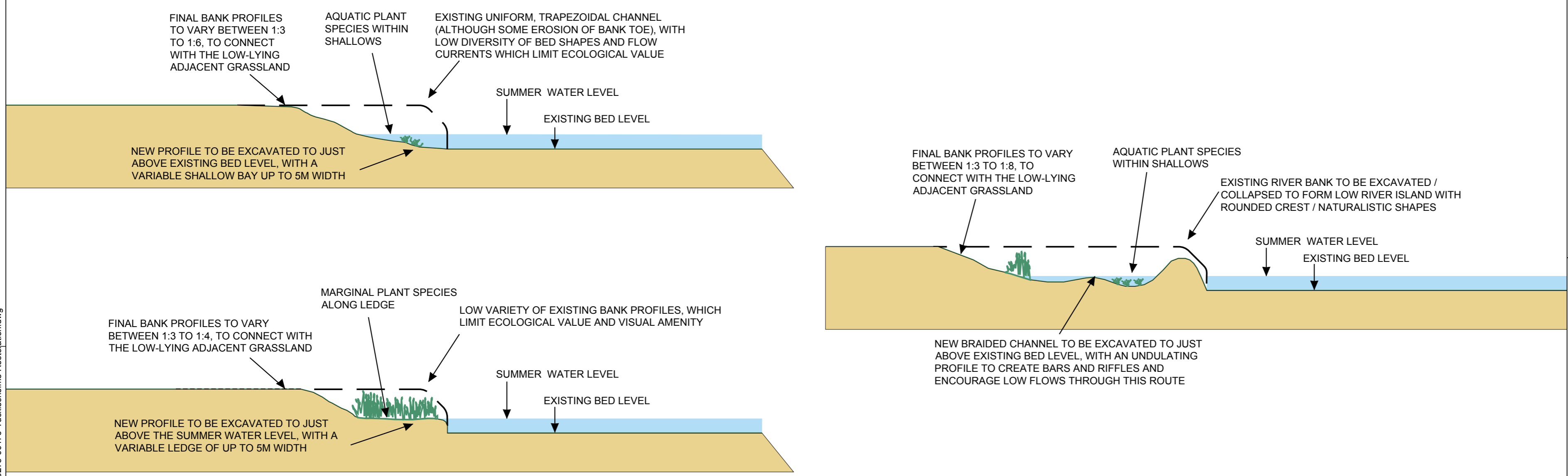
INDICATIVE SKETCH SECTIONS - NOT TO SCALE
